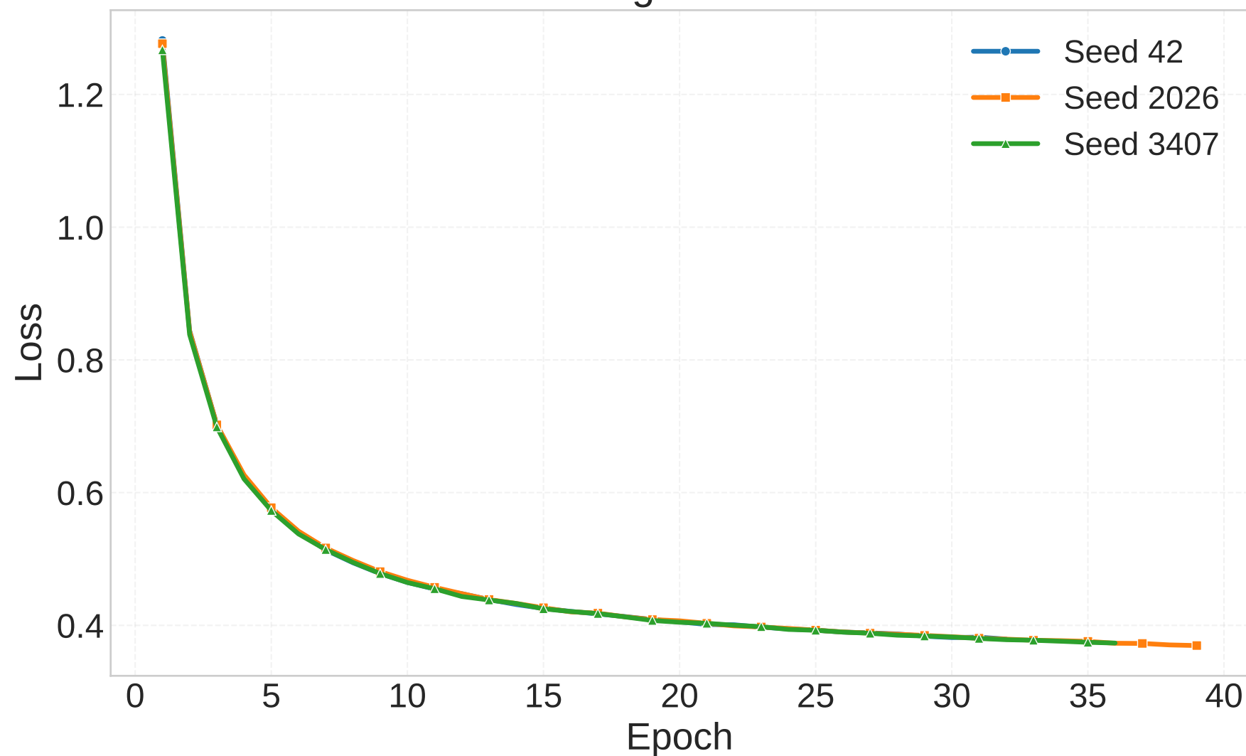
Training Total Loss
